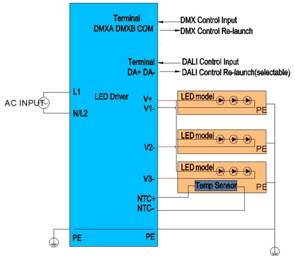
V1-, V2-, V3-cannot be connected together
