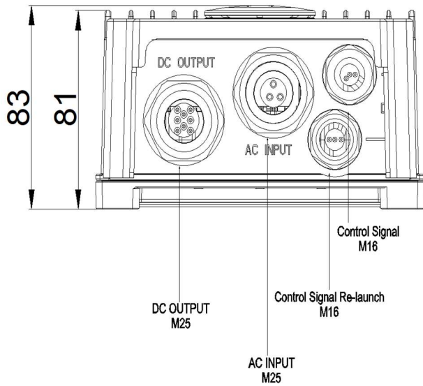
Wire Ports
