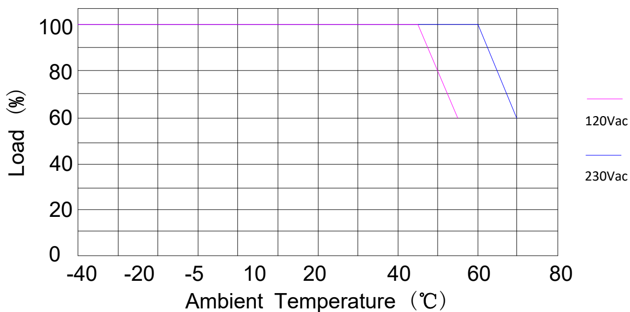
Derating Curve
