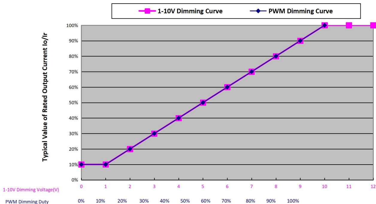
1-10V/PWM Dimming Curve
